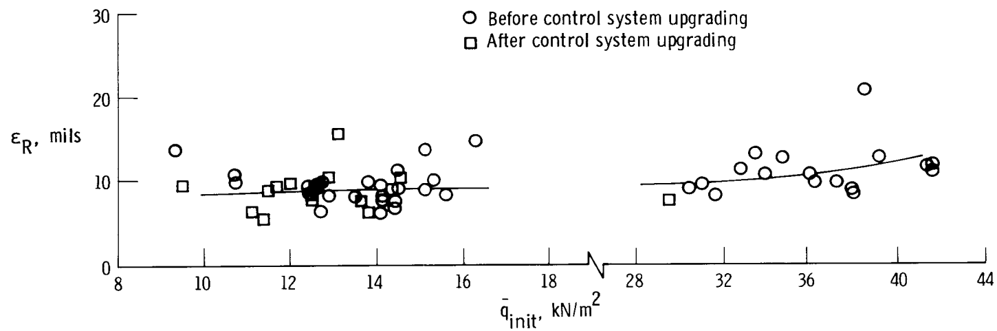
(b) Dynamic pressure.
