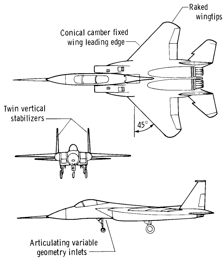
Figure 1. F-15 airplane.
